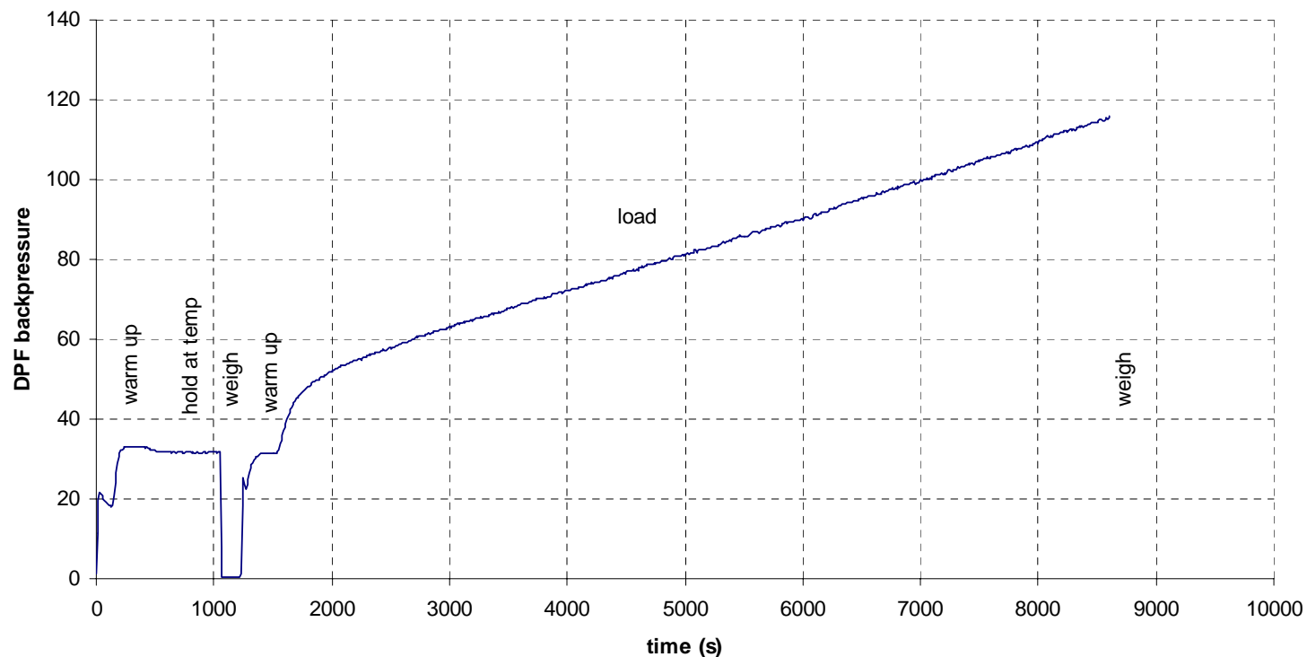
Loading test : Dp vs time
